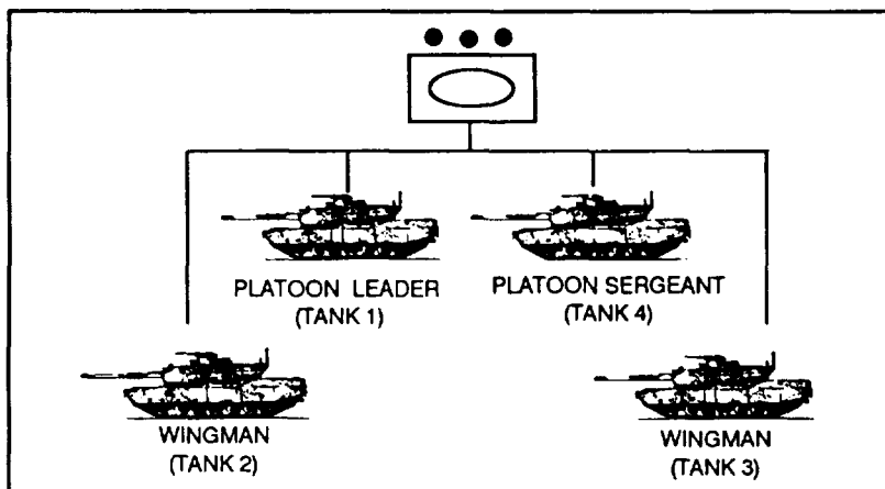
Figure 2-72. Tank platoon.
